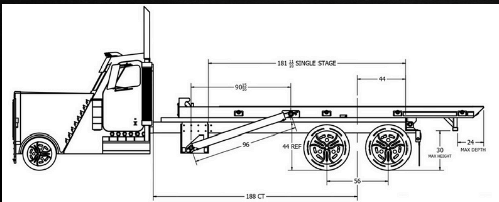
XOR Series Side Profile with Key Dimensions
